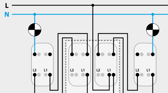
TWO-WAY SWITCH DOUBLE TWO-WAY SWITCH TWO-WAY SWITCH
