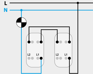
TWO-WAY SWITCH TWO-WAY SWITCH
