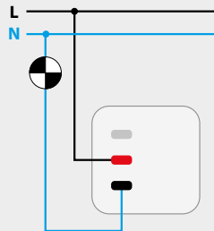
HOTEL CARD SWITCH, 1 MICROSWITCH - GARBY COLONIAL (37935...)
