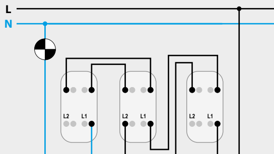
TWO-WAY SWITCH INTERMEDIATE SWITCH TWO-WAY SWITCH
