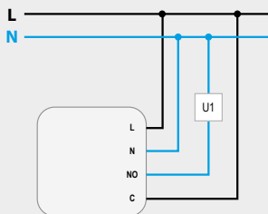
THERMOSTAT - 1950 (797300...)
