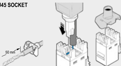
RJ45 SOCKET
