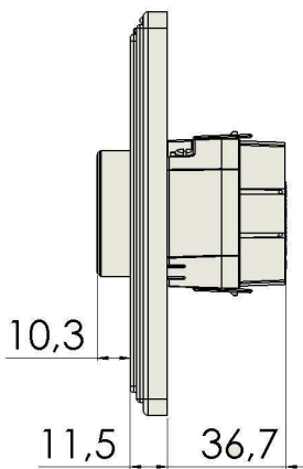
Height dimensions (size in mm)
